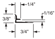
14289 1/16" Insert Cove FINISH: SS and SG
