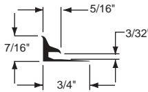
18176 3/32" Insert Cove FINISH: SS and SG
