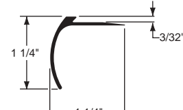
17353 For 3/32" Material FINISH: HT and HG
