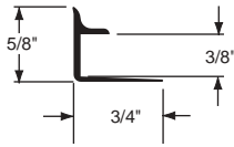
17134 Tile Cove FINISH: SS and SG
