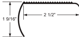
14294 Stair Tread FINISH: MB and SG
