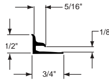
99951 1/8" Insert Cove FINISH: SS and SG
