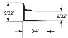
99929 Tile Cove FINISH: SS and SG
