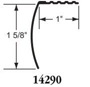
14290 FINISH: HT, HG, HB and GV
