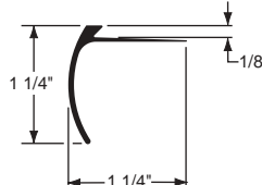
17352 For 1/8" Material FINISH: HT and HG
